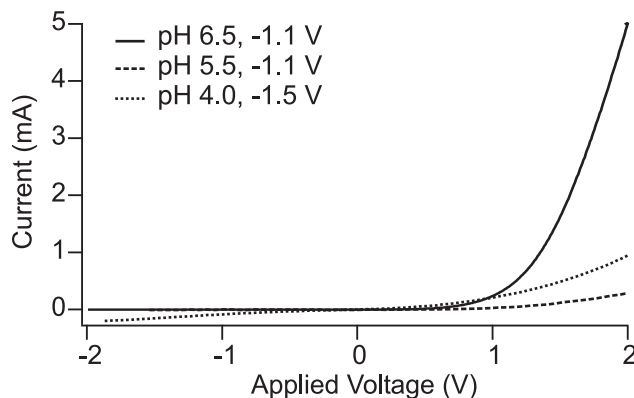
Figure 5: Representative I-V sweeps on electrodeposited ZnO Schottky junctions show stronger rectification and less soft breakdown with an increase in deposition electrolyte pH from 4.0 to 6.5. A representative I-V curve for pH 7.0 would coincide with the data for pH 6.5, so it is omitted for clarity.
