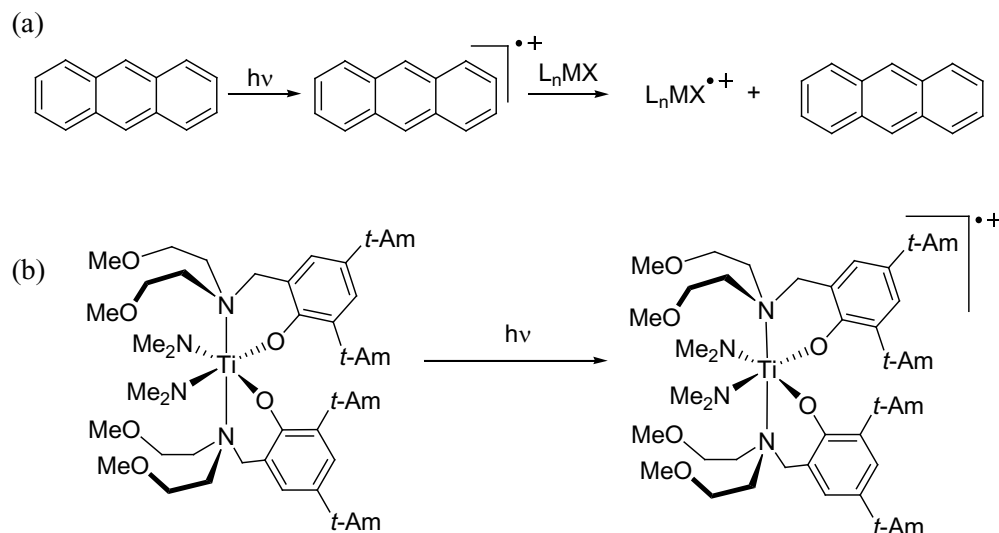
Scheme 1 (a) Ionization by charge-transfer in MALDI-TOF mass spectrometry with arene matrices, 4 (b) Proposed direct ionization in LDI-TOF of Ti-phenolate complexes, the radical is likely delocalised on the phenolate ligand and the positive charge on the metal center.
