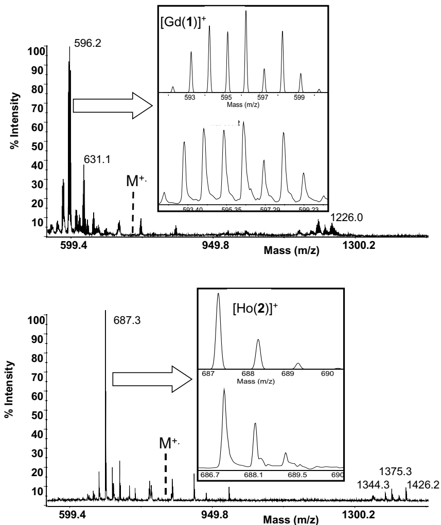
Figure 1. Mass spectra of isolated [1]GdN(SiMe 3 ) 2 and [2]HoN(SiMe 3 ) 2 , insets contain isotope patterns for the fragment [Ln(amine-phenolate)] + , simulated (top) and observed (bottom). Expected position of intact [Ln(amine-phenolate)N(SiMe 3 ) 2 ] + indicated by dotted line.
