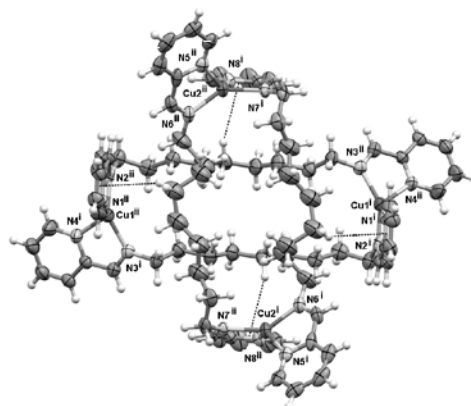
Figure 7. Dimer unit, [\text{Cu}_2(\text{L5})_2] , showing close methylene C-H... \pi interactions (30% probability ellipsoids); disordered carbon-chain atoms, \text{PF}_6^- ions and lattice solvent \text{CH}_3\text{OH} omitted for clarity.
