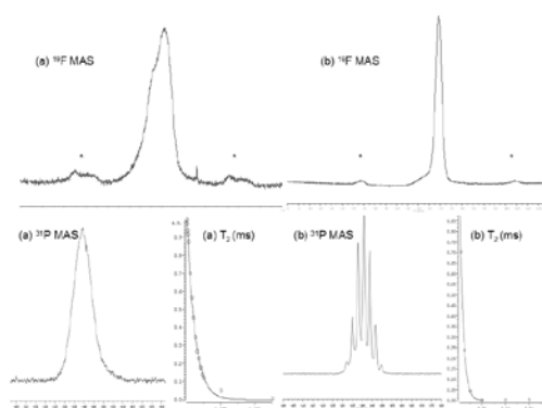
Figure 9. Solid-state NMR spectra for (a) [\text{Cu}(\text{L1})](\text{PF}_6) , ^{19}\text{F} -NMR \delta -65 (v.br) (deconvoluted as two environments \delta -67 (F1 35%), -60 (F2 65%), ^{31}\text{P} -NMR \delta -139 (v.br), J_{\text{F-P}} = 685\text{ Hz} , T_2 = 0.46\text{ ms} , T_2^* = 0.34\text{ ms} ; (b) [\text{Cu}(\text{L2})](\text{PF}_6) , ^{19}\text{F} -NMR \delta -70 (br), ^{31}\text{P} -NMR \delta -141 (septet), J_{\text{F-P}} = 711\text{ Hz} , T_2 = 2.81\text{ ms} , T_2^* = 1.26\text{ ms} . (* = spinning side bands).
