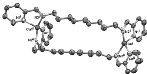
Figure 6. 30% probability ellipsoid representation of one of the two bimetallic moieties, \{\text{Cu}_2(\text{L5})_2\} (H-atoms omitted for clarity). Symmetry codes: (i) x, y, z (ii) x, 1.25-y, 1.25-z. Selected bond lengths [Å] and bond angles [°]: Cu1-N2 1.770(7); Cu1-N3 1.983(7); Cu1-N4 2.062(8); Cu1-N1 2.069(8); Cu2-N7 1.979(6); Cu2-N6 1.990(7); Cu2-N5 2.047(8); Cu2-N8 2.054(7) N2-Cu1-N3 140.9(3); N2-Cu1-N4 113.0(3); N3-Cu1-N4 80.9(3); N2-Cu1-N1 83.6(3); N3-Cu1-N1 119.2(3); N4-Cu1-N1 125.1(3); N7-Cu2-N6 140.6(3); N7-Cu2-N5 118.0(3); N6-Cu2-N5 82.1(3); N7-Cu2-N8 82.2(3); N6-Cu2-N8 112.2(3); N5-Cu2-N8 129.4(3).
