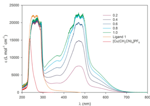
Figure 4. UV-Vis spectra for the titration of L1 with [\text{Cu}(\text{CH}_3\text{CN})_4](\text{PF}_6) in \text{CH}_2\text{Cl}_2 ; \text{Cu} = [\text{Cu}(\text{CH}_3\text{CN})_4](\text{PF}_6) only, \text{L1} = \text{L1} only, molar equiv. of Cu with respect to L1 from 0.2 to 1.0.
