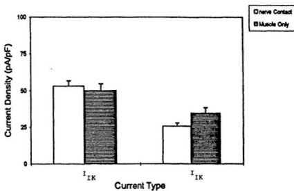
Figure 10: Effect of Nerve-Contact on Outward K + Current Density
