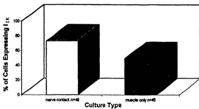
Figure 9a: Effect of Nerve-Contact on I_{IK} Expression
