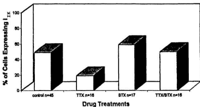
Figure 13b: Drug Effects on I_{IK} Expression in Muscle Only Cells
