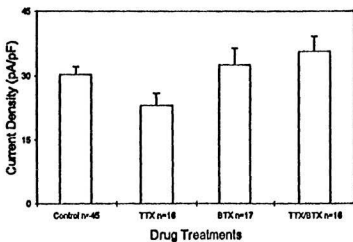
Figure 15b: Drug Effects on IR Current Density in Muscle Only Cells
