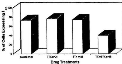
Figure 13a: Drug Effects on I_{IK} Expression in Nerve-Contacted Muscle Cells
