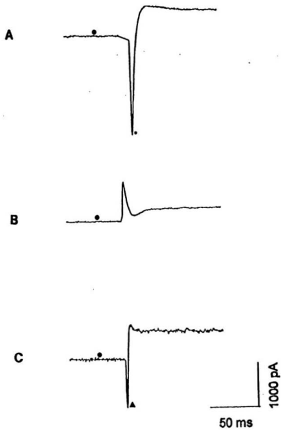
Figure 6: Acute Effect of TTX Treatment on I_{Na} Expression
