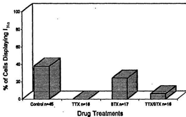
Figure 7b: Drug Effects on I_{Na} Expression in Muscle Only Cells
