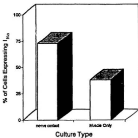
Figure 5: Effect of Nerve Contact on I_{Na} Expression
