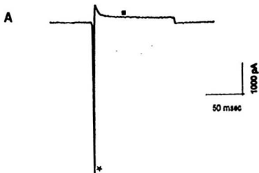
Figure 4: Sodium Trace From a Nerve-Contacted Muscle Cell
