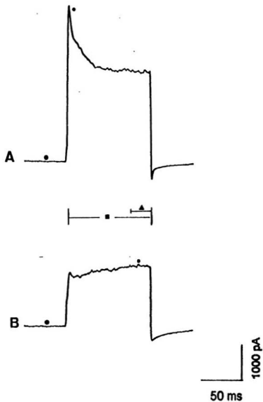
Figure 8: Outward K^+ Currents From Muscle Cells Cultured in the Absence of Nerve Cells
