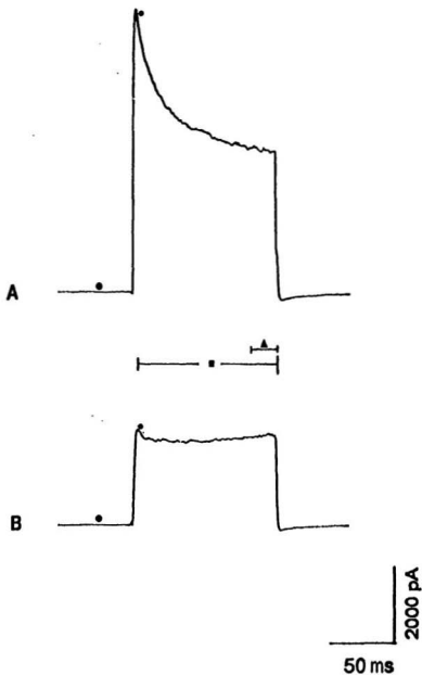
Figure 11: Outward K^+ Currents From Nerve-Contacted Muscle Cells
