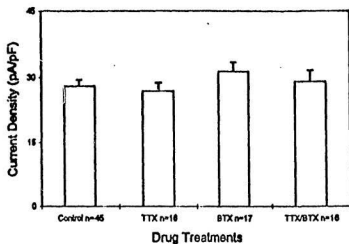
Figure 15b: Drug Effects on IR Current Density in Muscle Only Cells
