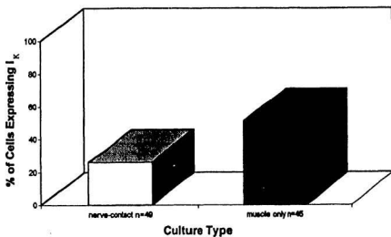
Figure 9b: Effect of Nerve-Contact on I_K Expression
