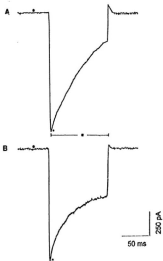
Figure 14: Inward Rectifier Current Traces in Muscle Only and Nerve-Contacted Muscle Cells
