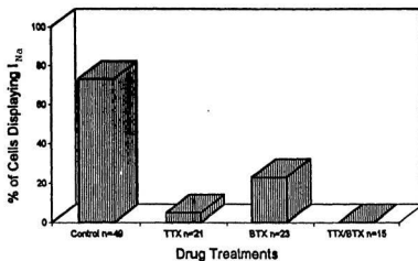
Figure 7a: Drug Effects on I_{Na} Expression in Nerve-Contacted Muscle Cells
