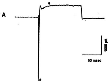
Figure 3: Sodium Current Trace Recorded From a Muscle Cell in a Culture Which Contained no Nerve Cells.
