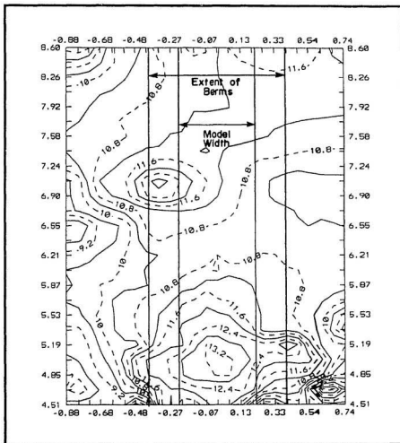
Figure 6.18: Penetration Resistance of the Testbed, Test 3.
