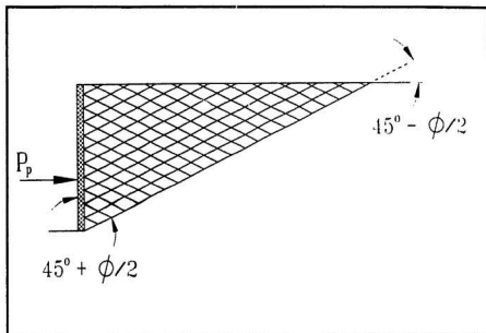
Figure 2.14: Rankine Earth Pressure Passive Failure Surface (After Craig, 1987).
