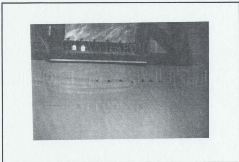
Figure 6.3: Front Failure Surface During Scour.
