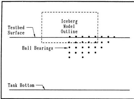
Figure 5.4: Ball Bearing Locations, X-Z Plane.
