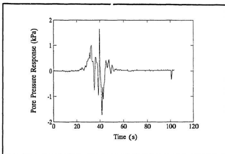
Figure 6.12: Pore Pressure Transducer #6 Response vs. Time, Test 3.
