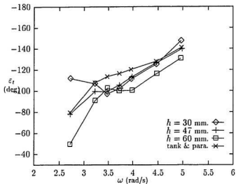
Figure 4.15: Phase lags of undamped tank, \omega_\phi = 3.75 , h_w = 10
