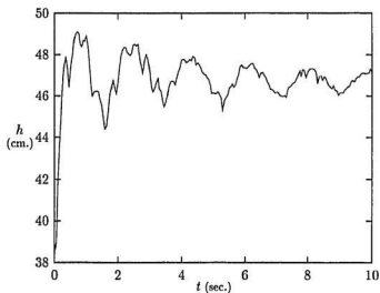
Figure 2.8: A tank decay test for obtaining natural frequency
