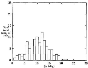
Figure 5.14: Histogram of unstabilized roll
