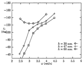
Figure 4.18: Phase lags of undamped tank, \omega_\phi = 3.00 , h_w = 5
