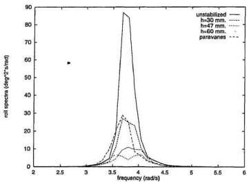
Figure 5.8: Roll spectra for damped tank, \omega_\phi = 3.75 , (h_w)_{1/3} = 4.4
