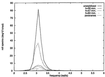
Figure 5.12: Roll spectra for damped tank, \omega_\phi = 3.00 , (h_w)_{1/3} = 4.7
