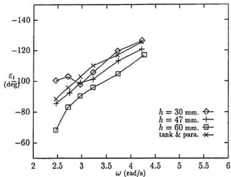
Figure 4.7: Phase lags of damped tank, \omega_\phi = 3.00 , h_w = 10
