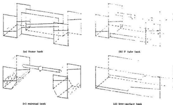
Figure 1.1: Common configurations of passive tanks
