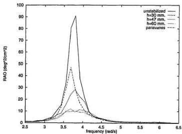
Figure 5.9: RAOs for damped tank, \omega_\phi = 3.75 , (h_w)_{1/3} = 4.4
