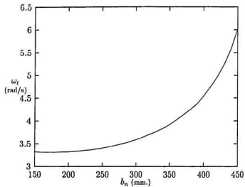
Figure 2.4: \omega_t vs. b_n , l_t = 85 , l_n = 40 , h = 50
