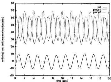
Figure 2.9: Showing tank-water elevations and roll motions
