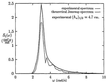
Figure 5.4: Wave spectra for \omega_0 = 3.00 and (h_w)_{1/3} = 5
