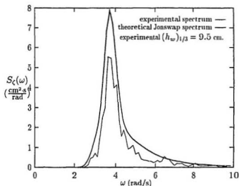
Figure 5.1: Wave spectra for \omega_0 = 3.75 and (h_w)_{1/3} = 10
