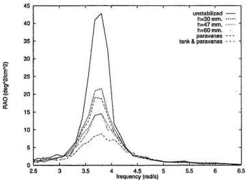
Figure 5.7: RAOs for damped tank, \omega_\phi = 3.75 , (h_w)_{1/3} = 9.5
