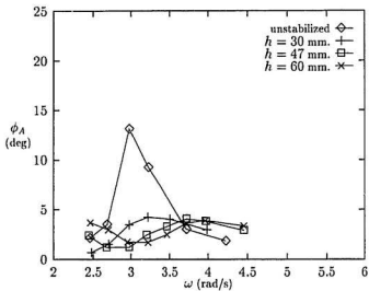
Figure 4.12: Roll response of M366 with undamped tank, \omega_\phi = 3.00 , h_w = 5
