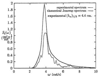
Figure 5.2: Wave spectra for \omega_0 = 3.75 and (h_w)_{1/3} = 5
