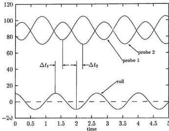
Figure 2.10: Fits of tank-water elevations and roll motions
