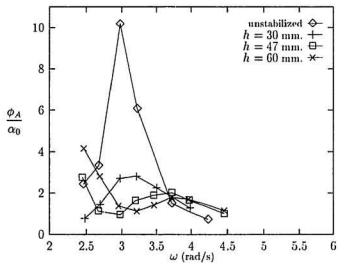
Figure 4.14: Amplification factor at \omega_\phi = 3.00 , h_w = 5
