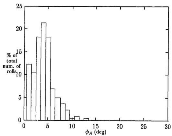
Figure 5.15: Histogram of stabilized roll
