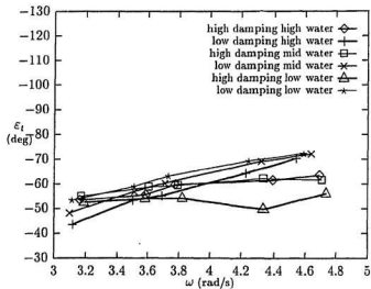
Figure 2.13: \varepsilon_t , bench tests for l_t = 68 mm.
