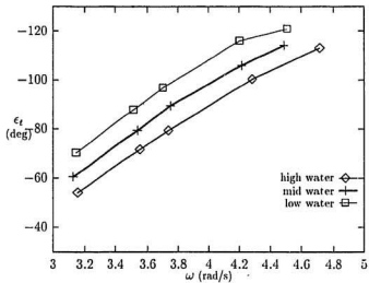
Figure 2.19: \epsilon_t of the modified tank without damping
