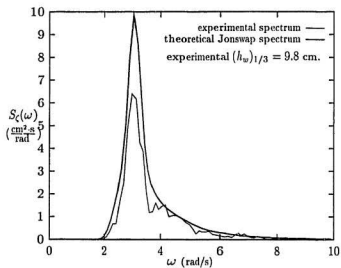
Figure 5.3: Wave spectra for \omega_0 = 3.00 and (h_w)_{1/3} = 10
