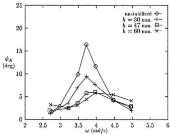
Figure 4.10: Roll response of M366 with undamped tank, \omega_\phi = 3.75 , h_w = 5
