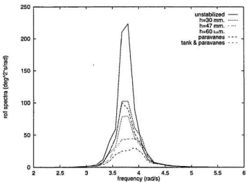
Figure 5.6: Roll spectra for damped tank, \omega_\phi = 3.75 , (h_w)_{1/3} = 9.5
