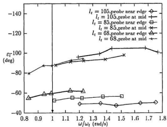
Figure 2.15: Comparison of different probe positions with high damping
