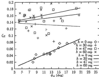
Figure 3.5: \zeta_E of M36G, tank with damping, \omega_\phi = 3.00
