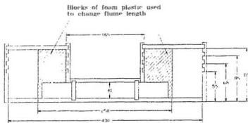
Figure 2.6: Configurations of the tank model
