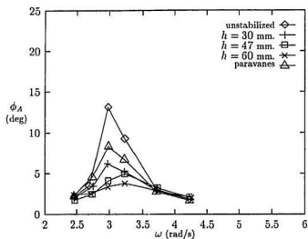
Figure 4.4: Roll response of M366 with damped tank, \omega_\phi = 3.00 , h_w = 5
