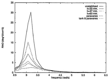
Figure 5.11: RAOs for damped tank, \omega_\phi = 3.00 , (h_w)_{1/3} = 9.8
