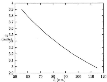
Figure 2.2: \omega_t vs. l_t , l_n = 40 , b_n = 220 , h = 50
