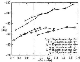
Figure 2.16: Comparison of different probe positions with low damping
