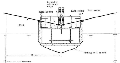
Figure 3.3: Experimental setup
