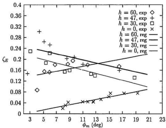
Figure 3.7: \zeta_E of M366, tank without damping, \omega_\phi = 3.00
