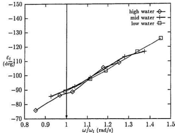
Figure 2.18: \varepsilon_t vs. nondimensional frequency, modified tank with damping
