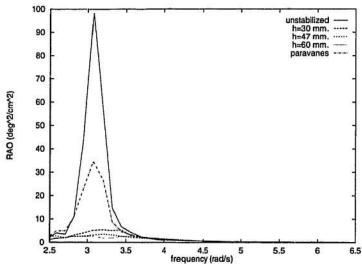
Figure 5.13: RAOs for damped tank, \omega_\phi = 3.00 , (h_w)_{1/3} = 4.7
