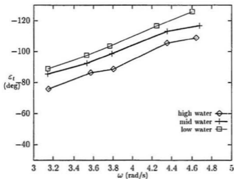
Figure 2.17: \varepsilon_t of the modified tank with damping
