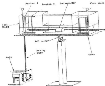
Figure 2.7: Oscillating bench test setup
