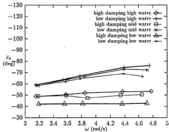
Figure 2.11: \varepsilon_t , bench tests for l_t = 105 mm.
