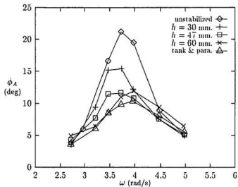
Figure 4.9: Roll response of M366 with undamped tank, \omega_\phi = 3.75 , h_w = 10
