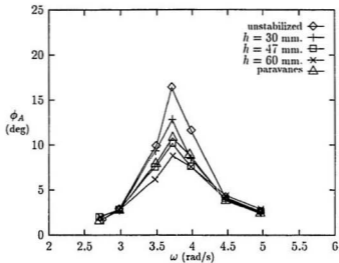
Figure 4.2: Roll response of M366 with damped tank, \omega_\phi = 3.75 , h_w = 5
