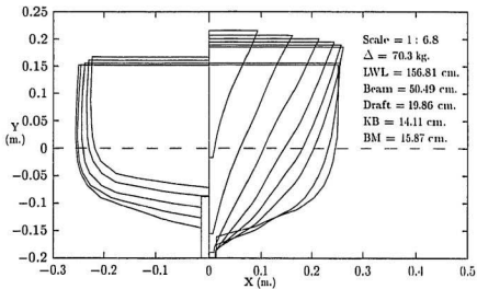
Figure 3.1: Body plan and particulars of Model 366
