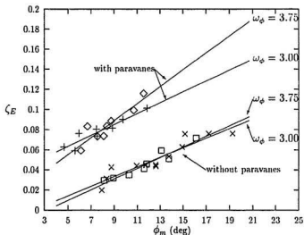
Figure 3.8: \zeta_E of M366 with paravanes
