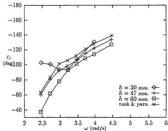
Figure 4.17: Phase lags of undamped tank, \omega_\phi = 3.00 , h_w = 10
