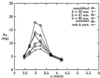
Figure 4.3: Roll response of M366 with damped tank, \omega_\phi = 2.00 , h_w = 10
