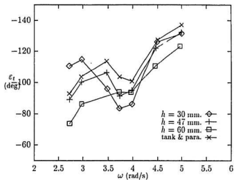
Figure 4.5: Phase lags of damped tank, \omega_\phi = 3.75 , h_w = 10
