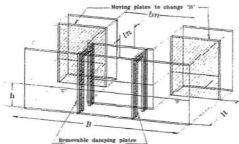
Figure 2.1: Tank Model
