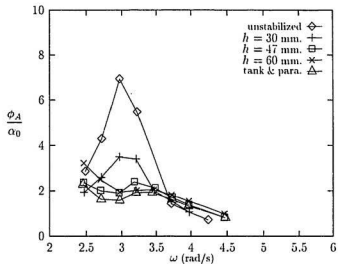
Figure 4.13: Amplification factor at \omega_\phi = 3.00 , h_w = 10
