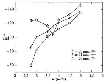
Figure 4.6: Phase lags of damped tank, \omega_\phi = 3.75 , h_w = 5
