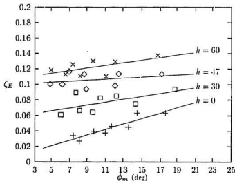
Figure 3.4: \zeta_E of M366, tank with damping, \omega_\phi = 3.75
