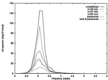
Figure 5.10: Roll spectra for damped tank, \omega_\phi = 3.00 , (h_w)_{1/3} = 9.8
