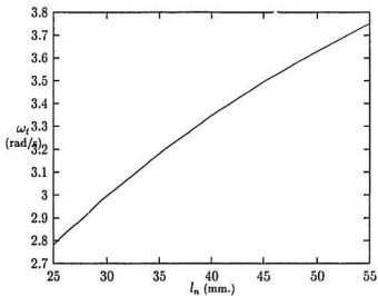
Figure 2.3: \omega_t vs. l_n , l_t = 85 , b_n = 220 , h = 50
