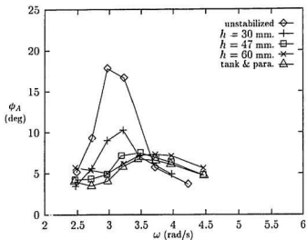
Figure 4.11: Roll response of M366 with undamped tank, \omega_\phi = 3.00 , h_w = 10
