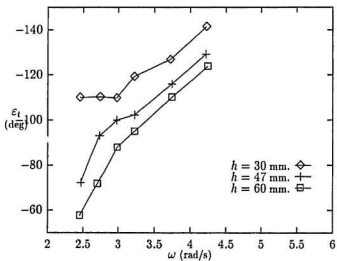
Figure 4.8: Phase lags of damped tank, \omega_\phi = 3.00 , h_w = 5
