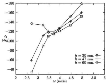
Figure 4.16: Phase lags of undamped tank, \omega_\phi = 3.75 , h_w = 5
