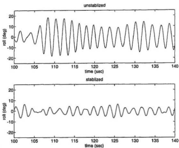
Figure 5.5: Roll samples for irregular wave tests
