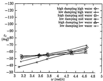
Figure 2.14: \varepsilon_t , bench tests for l_t = 55 mm.
