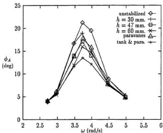
Figure 4.1: Roll response of M366 with damped tank, \omega_\phi = 3.75 , h_w = 10
