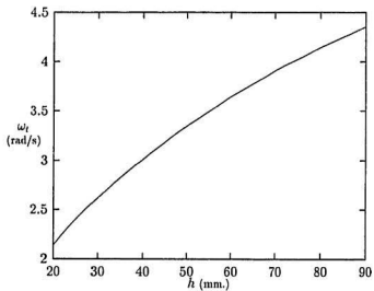
Figure 2.5: \omega_t vs. h , l_t = 85 , l_n = 40 , b_n = 220
