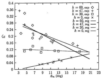
Figure 3.6: \zeta_E of M366, tank without damping, \omega_\phi = 3.75
