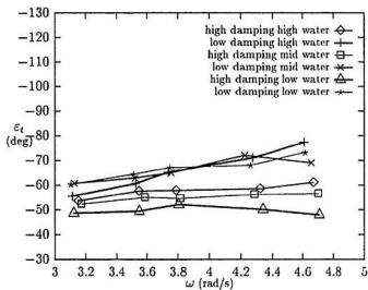
Figure 2.12: \varepsilon_t , bench tests for l_t = 85 mm.
