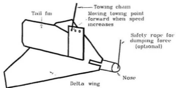
Figure 1.2: The shape of a paravane
