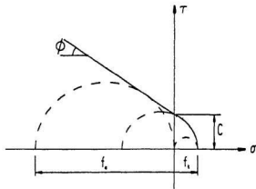
a) Modified Coulomb failure criterion
