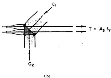
Figure 3.5: Tension tie and reinforcement [48].
