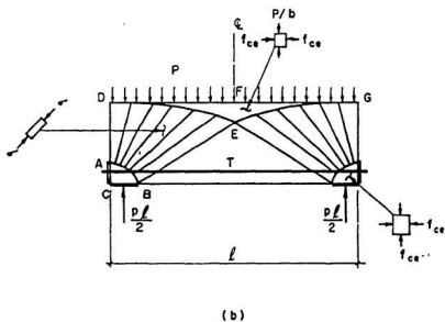
Figure 3.11: Parabolic decentered fan and application [48].
