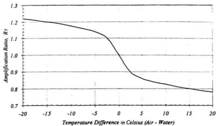
Figure 3.2: Stability Ratio, R_T (Resio and Vincent, 1977)
