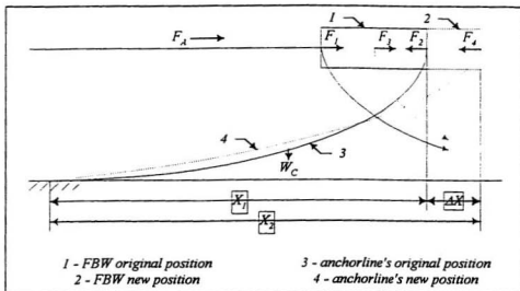
Figure 4.1: Catenary Mooring System
