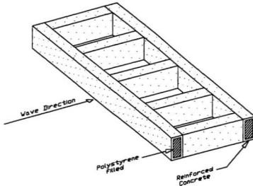
Figure 2.5: Alaskan Floating Breakwater
