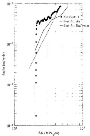
Figure A.2: Neutrient test: specimen one
