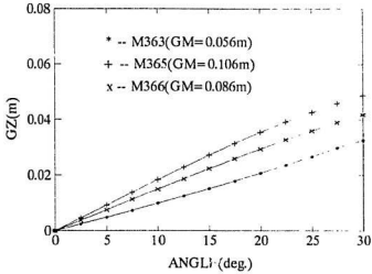
Figure 2.7: GZ curves for three models
