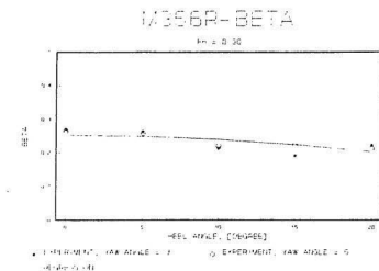
Figure 15(b) \beta vs. \varphi for M366R at Fn = 0.30
