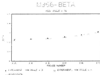
Figure C6 \beta vs. F_n for M366 at \varphi = 10^\circ
