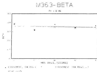
Figure G5 \beta vs. \varphi for M363 at Fn = 0.46
