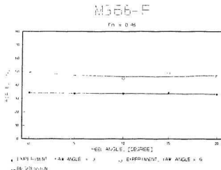
Figure E10 Force vs. \varphi for M366 at Fn = 0.46
