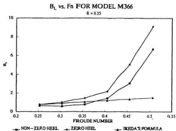
Figure 22 B_L vs. F_n for M366 with R=0.35
