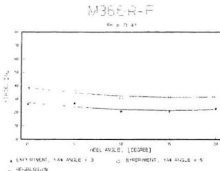
Figure E14 Force vs. \varphi for M366R at F_n = 0.41
