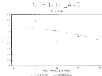
Figure 16(e) L/T vs. \varphi for M363 at Fn = 0.46
