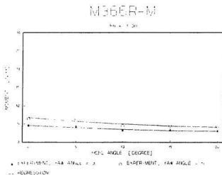
Figure F12 Moment vs. \phi for M366R at F_n = 0.30
