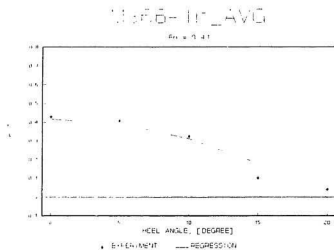
Figure 17(d) I_r/T vs. \varphi for M366 at Fn = 0.41
