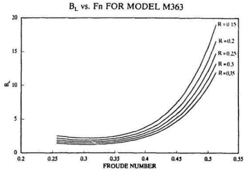
Figure 20(a) B_L vs. Fn for M363 at different R values
