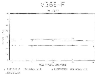
Figure E9 Force vs. \varphi for M366 at Fn = 0.41
