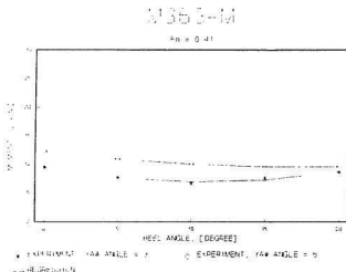
Figure F4 Moment vs. \varphi for M363 at Fn = 0.41
