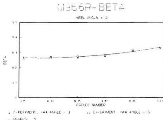
Figure 10(c) \beta vs. Fn for M366R in upright condition
