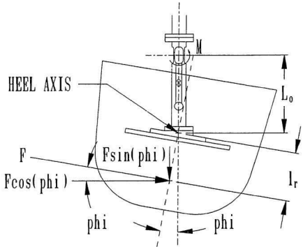
Figure 7 Free body diagram for the ship model in a fixed heel angle
