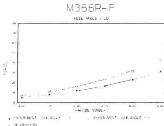
Figure A12 Force vs. F_n for M366R at \varphi = 20^\circ
