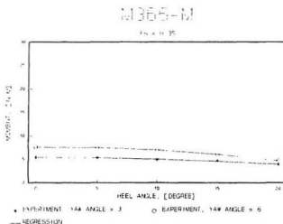
Figure F8 Moment vs. \varphi for M366 at Fn = 0.35
