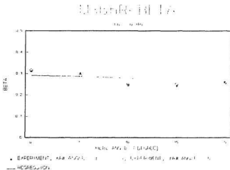
Figure 15(e) \beta vs. \varphi for M366R at Fn = 0.46
