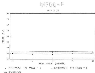
Figure E6 Force vs. \varphi for M366 at F_n = 0.25
