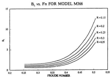
Figure 20(b) B_L vs. F_n for M366 at different R values
