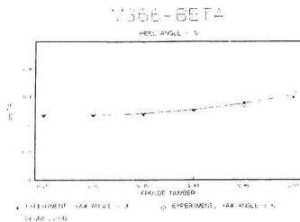
Figure C5 \beta vs. F_n for M366 at \varphi = 5^\circ
