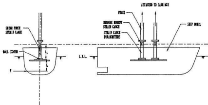
Figure 2 Equipment arrangement
