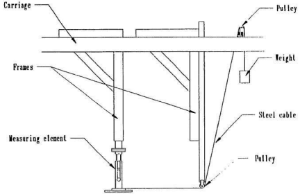
Figure 6 Calibration setup
