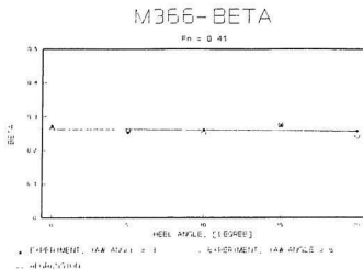
Figure G9 \beta vs. \varphi for M366 at F_n = 0.41
