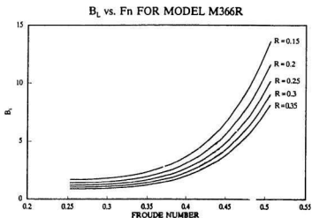
Figure 20(c) B_L vs. F_n for M366R at different R values
