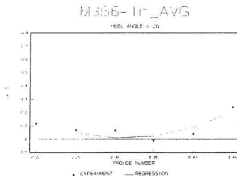
Figure D8 I_r/T vs. F_n for M366 at \varphi = 20^\circ
