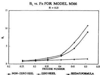
Figure 24 B_L vs. F_n for M366 with R=0.25
