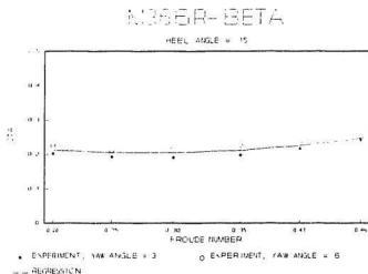
Figure 13(c) \beta vs. F_n for M366R at \varphi = 15^\circ
