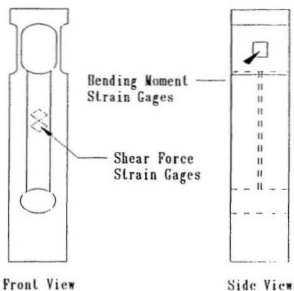
Figure 1 Measuring element
