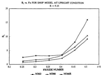
Figure 12 B_L vs. F_n for models M363, M366 and M366R in upright condition
