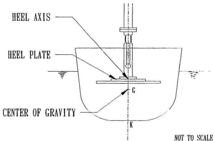
Figure 5 Positions of heel axis and center of gravity
