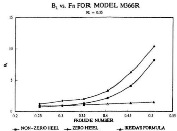
Figure 23 B_L vs. F_n for M366R with R=0.35
