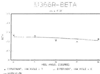
Figure 15(c) \beta vs. \varphi for M366R at Fn = 0.35
