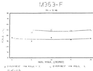
Figure E5 Force vs. \varphi for M363 at F_n = 0.46
