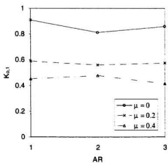
Figure 7.7 Comparison of earth pressure coefficient at-rest, K_{0,1} , and the associated aspect ratio, AR, for contact friction, \mu = 0, 0.2 and 0.4 : gravity method
