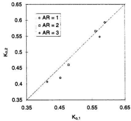
Figure 7.12 Comparison of the at-rest earth pressure coefficient, K_{o,2} , in simulated oedometer tests and the corresponding coefficient, K_{o,1} , estimated from gravity test simulations
