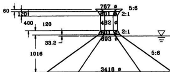
Figure 3.4 Dimensions of the 1:50 large neck model. All diameters are corner to corner; all slopes are of the facet centres and given as a ratio of vertical to horizontal. All dimensions in millimetres.
