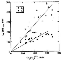
Figure 2.4 Piece size, L_w and L_L , versus the parameter, (\sigma_t/\gamma_w)^{0.5} , for IME's tests (after Izumiyama et al, 1994)
