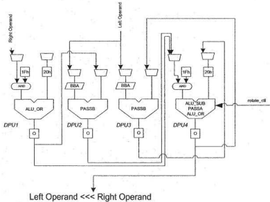
Figure 4.7: Four DPU implementation of the data dependent rotation.
