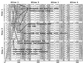
Figure 4.5: C~SIDE floorplanner screen shot of simple iterative RC5 design.
