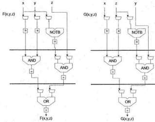
Figure 5.1: Implementation of F and G functions.
