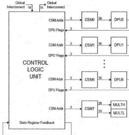
Figure 3.15: CLU communication and interaction with processing elements.
