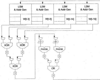
Figure 5.4: Recursive expansion of W[0..15] to W[0..79] .
