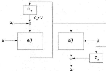
Figure 2.3: CBC mode.
