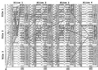
Figure 4.19: RC6 pipeline floorplan.
