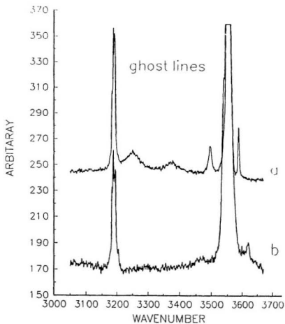
Figure 4.5. Raman Spectra ( 3000\text{--}3650\text{ cm}^{-1} ) of Precipitates from (a) the Potassium Aluminate Solutions and (b) the Sodium Aluminate Solutions
