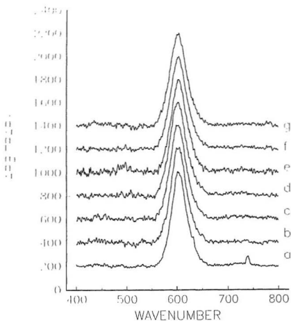
Figure 5.3. Raman Spectra ( 400\text{--}800\text{ cm}^{-1} ) of \text{Al}(\text{OH})_4^- in \text{H}_2\text{O} at (a) 25^\circ\text{C} , (b) 50^\circ\text{C} , (c) 75^\circ\text{C} , (d) 100^\circ\text{C} , (e) 115^\circ\text{C} , (f) 130^\circ\text{C} and (g) 150^\circ\text{C}
