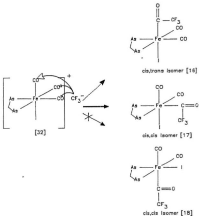
Figure 4.10: The Intermolecular Nucleophilic Addition in [\text{Fe}(\text{CO})_3(\text{diars})]\text{I}^+[\text{CF}_3]^-
