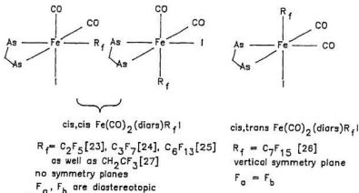
Figure 3.1: Structures of the Perfluoroalkyl Compounds
