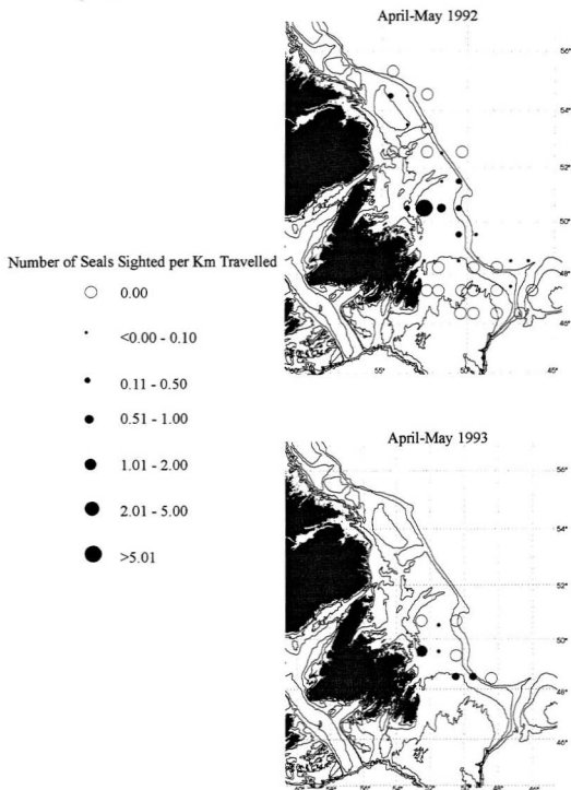
Figure 2.4. Annual relative sighting rates for harp seals standardized to 1 km effort in surveys conducted under fair to excellent sighting conditions for the April-May period.
