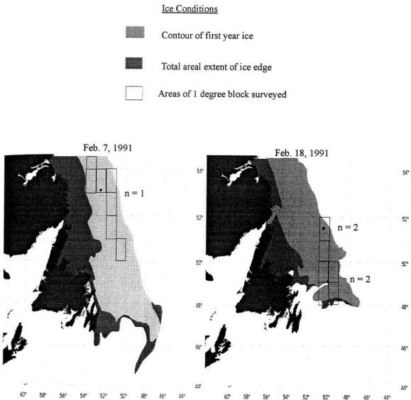
Figure 3.1. Winter 1991: Distribution of seals (black dots) in relation to ice conditions; n = number of seals.
