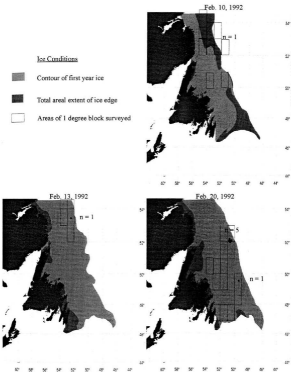
Figure 3.2. Winter 1992: Distribution of seals (black dots) in relation to ice conditions; n=number of seals.
