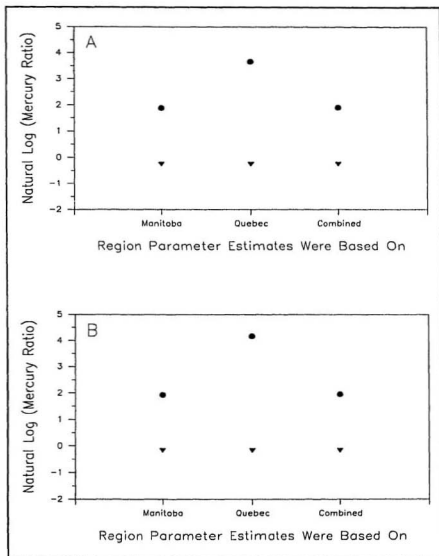
Figure 40 Predicted (•) and observed (▼) values of the natural log of the mercury ratio for Long Pond ouaniche using Model II for: (A) first sampling following reimpoundment; and (B) peak mercury concentration.
