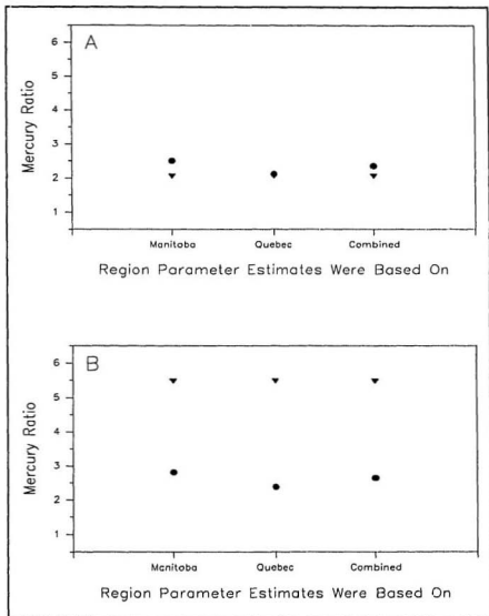
Figure S2 Predicted (●) and observed (▼) values of the mercury ratio for Arctic char in Cat Arm Reservoir using Model III for: (A) the first sampling following impoundment; and (B) the peak mercury concentration.
