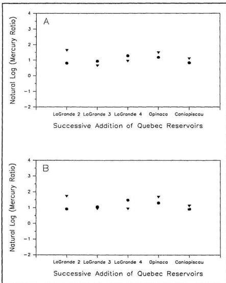
Figure 29 Predicted (•) and observed (▼) values of the natural logarithm of the mercury ratio for lake whitefish, for Model II using: (A) the first sampling period following impoundment; and (B) the peak mercury concentrations.
