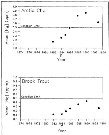
Figure 17 Mean mercury concentrations of Arctic char and brook trout sampled in Cat Arm Reservoir. The year of flooding (F) and the Canadian consumption guideline of 0.5 ppm mercury are shown.
