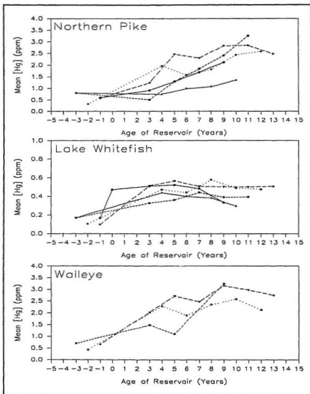
Figure 16 Mean mercury concentrations plotted against reservoir age for northern pike, walleye and lake whitefish for Caniapiscou (●); La Grande 2 (▼); La Grande 3 (■); La Grande 4 (▲); and Opinaca (◆) Reservoirs.
