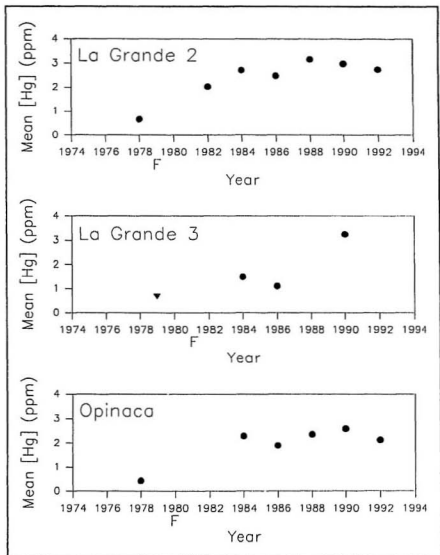
Figure 13 Mean mercury concentrations of walleye sampled from La Grande Complex reservoirs. Control lakes (▼) were used as a baseline when necessary. Year of flooding (F) is also indicated.
