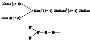
Fig. 2. The common core of N-linked oligosaccharides
