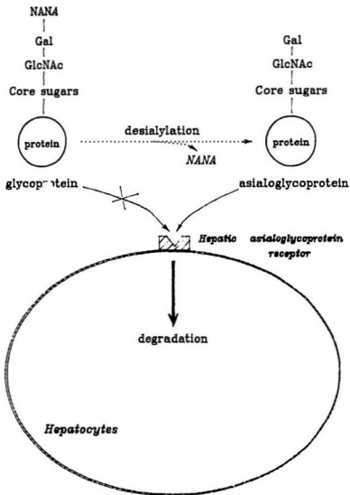
Fig. 4. Ashwell's pathway
