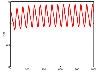
(3-2) \mathcal{R}_0 < 1
