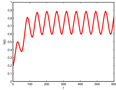
(4-2) R_0 < 1
