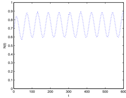
(4-1) R_0 > 1
