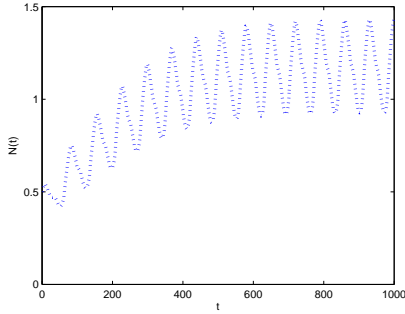
(3-1) \mathcal{R}_0 > 1
