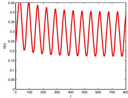
(1-2) R_0 < 1
