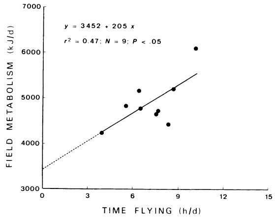
FIG. 1. Field metabolic rate as a function of mean daily time spent flying for nine Northern Gannets breeding at Funk Island, Newfoundland.
