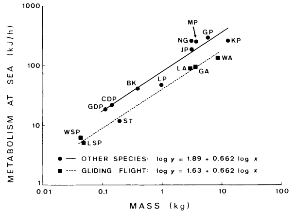
FIG. 3. Allometry of metabolic rates at sea for 15 seabird species, studied with tritiated (King Penguin) or doubly labeled (all others) water. Regression lines from ANCOVA (Table 4). See Table 1 for species symbols and references.
