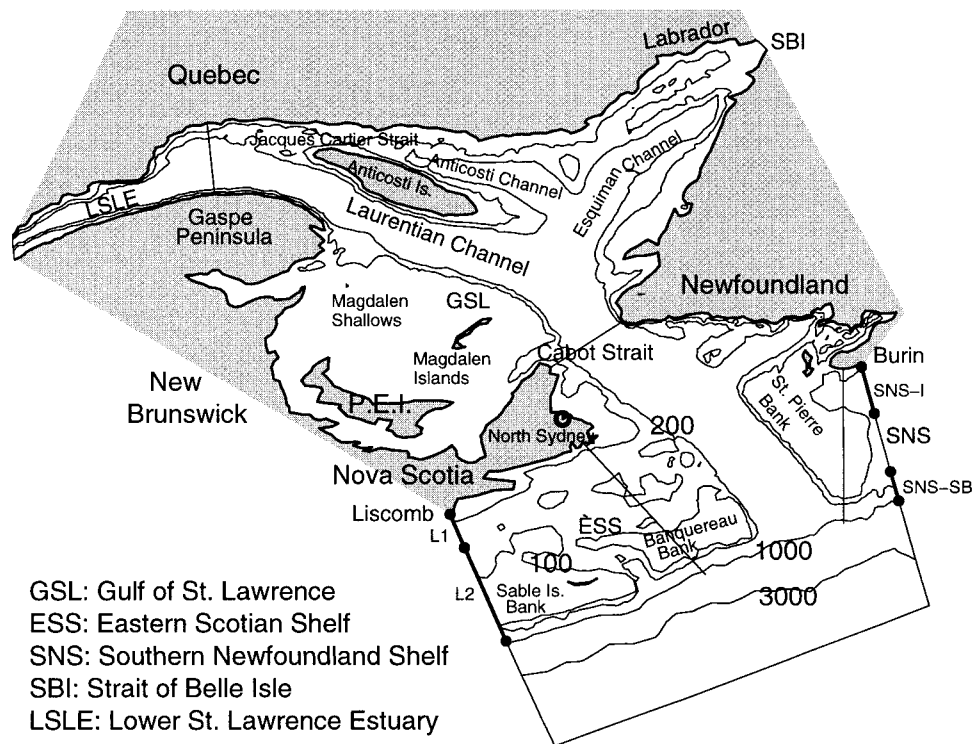
FIG. 1. Map showing the study domain, bathymetry, and section locations; isobaths shown are 100, 200, 1000, and 3000 m. The Gaspé, Cabot Strait, Burin, and Banquereau sections are shown in solid lines. SNS-I and SNS-SB are the inner and shelf-break segments of the upstream SNS boundary. L1 and L2 are the inner and outer segments of the Liscomb line on the downstream ESS boundary.
