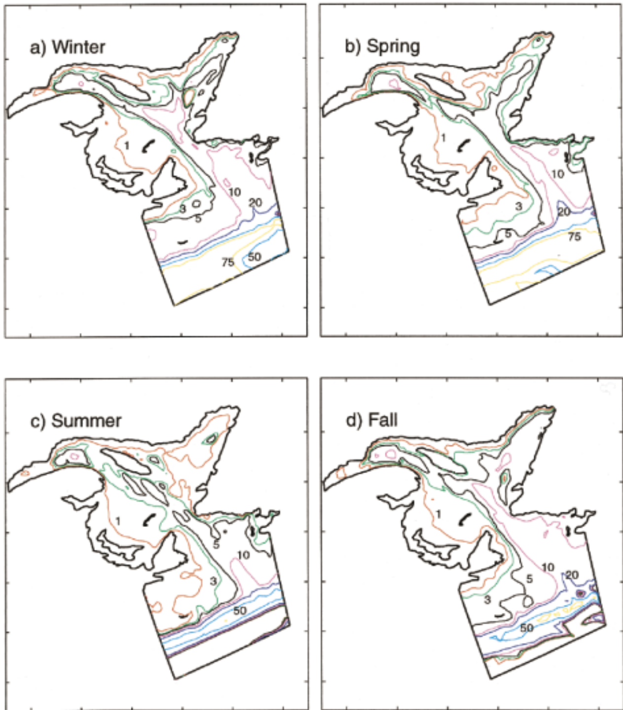
FIG. 10. Transport streamfunction in units of deci-Sv ( 10^5 \text{ m}^3 \text{ s}^{-1} ) for (a) winter, (b) spring, (c) summer, and (d) fall from the composite base model solutions. The forcing are baroclinic pressure gradients, wind stresses, and steric boundary conditions, except for additional flow components on the SBI, SNS, and ESS boundaries (as discussed in the text). The streamfunction value is zero along the Nova Scotia coast and the south and north shores of the gulf, with low values on the right looking downstream; that is, the flow is cyclonic around local streamfunction maxima and anticyclonic around local minima. The streamfunction values are 3, 2, 1, and 5 deci-Sv along the Newfoundland coast.
