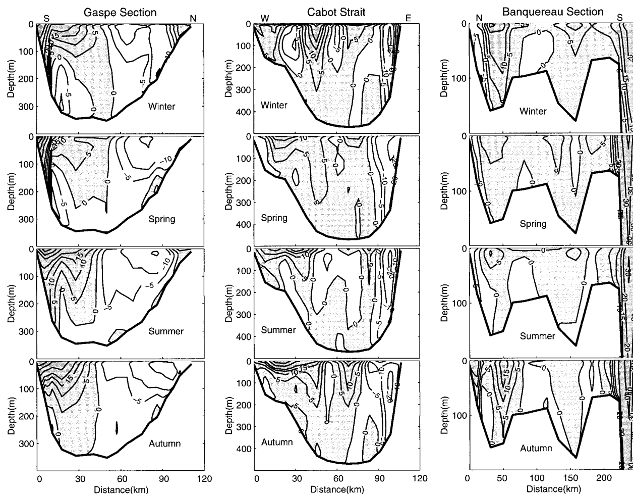
FIG. 12. Mean normal velocity on the Gaspé, Cabot Strait, and Banquereau sections for winter, spring, summer, and fall from the model solutions. The isotach interval is 5 \text{ cm s}^{-1} for currents between -10 and 20 \text{ cm s}^{-1} , 10 \text{ cm s}^{-1} for values below -10 \text{ cm s}^{-1} , or between 20 and 50 \text{ cm s}^{-1} , and 25 \text{ cm s}^{-1} for values above 50 \text{ cm s}^{-1} . Positive values (shaded) indicate eastward currents on the Gaspé section, seaward currents through Cabot Strait, and southeastward currents on the Banquereau section.
