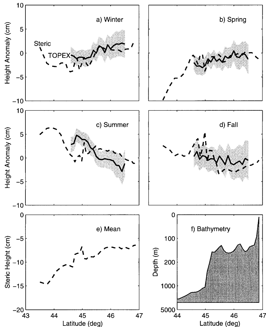
FIG. 9. Seasonal sea level anomalies along the SNS boundary for (a) winter, (b) spring, (c) summer, and (d) fall. Dashed lines are steric height estimates computed from the seasonal density field along the boundary, and solid lines are TOPEX/Poseidon altimetry data for 1992–96 with the gray shading indicating the standard error (Han and Smith 1997). The variations in annual-mean steric height and bottom topography along the boundary are shown in (e) and (f). See Fig. 7a for the TOPEX/Poseidon track location.
