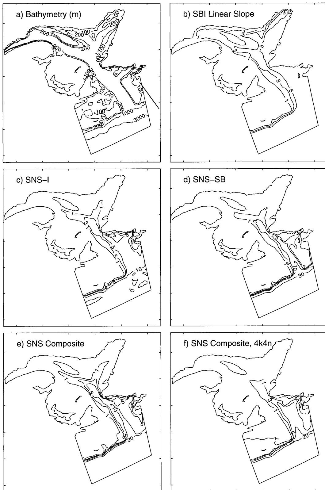
FIG. 7. (Continued) from the nonlinear M_2 tidal solution are used in (b)–(e). The streamlines are labeled in units of \text{dec-Sv} ( 10^5 \text{ m}^3 \text{ s}^{-1} ), with a value of zero specified on the Labrador [in (b)] or Newfoundland [in (c)–(f)] coast, and low values on the right looking downstream. The regional bathymetry is shown in (a) using the 100-, 200-, 1000-, and 3000-m isobaths. The thicker line crossing the SNS boundary in (a) shows the location of the TOPEX/Poseidon track used in Fig. 9.
