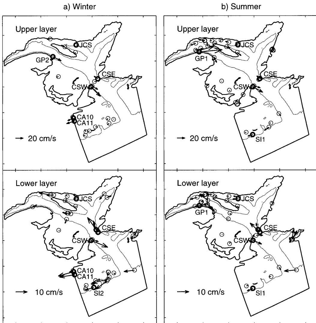
FIG. 4. Bimonthly mean currents from moored measurements for the upper layer (within 30 m of surface) and lower layer (remainder of the water column), computed by vertical averaging for (a) winter and (b) summer. For clarity, only representative data are shown. The 200-m isobath is included.
