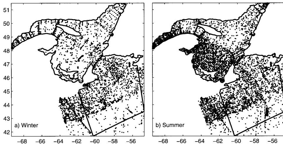
FIG. 2. The distribution of observational density data is in the depth interval 5–25 m for 6-month periods encompassing (a) winter (Nov–Apr) and (b) summer (May–Oct).
