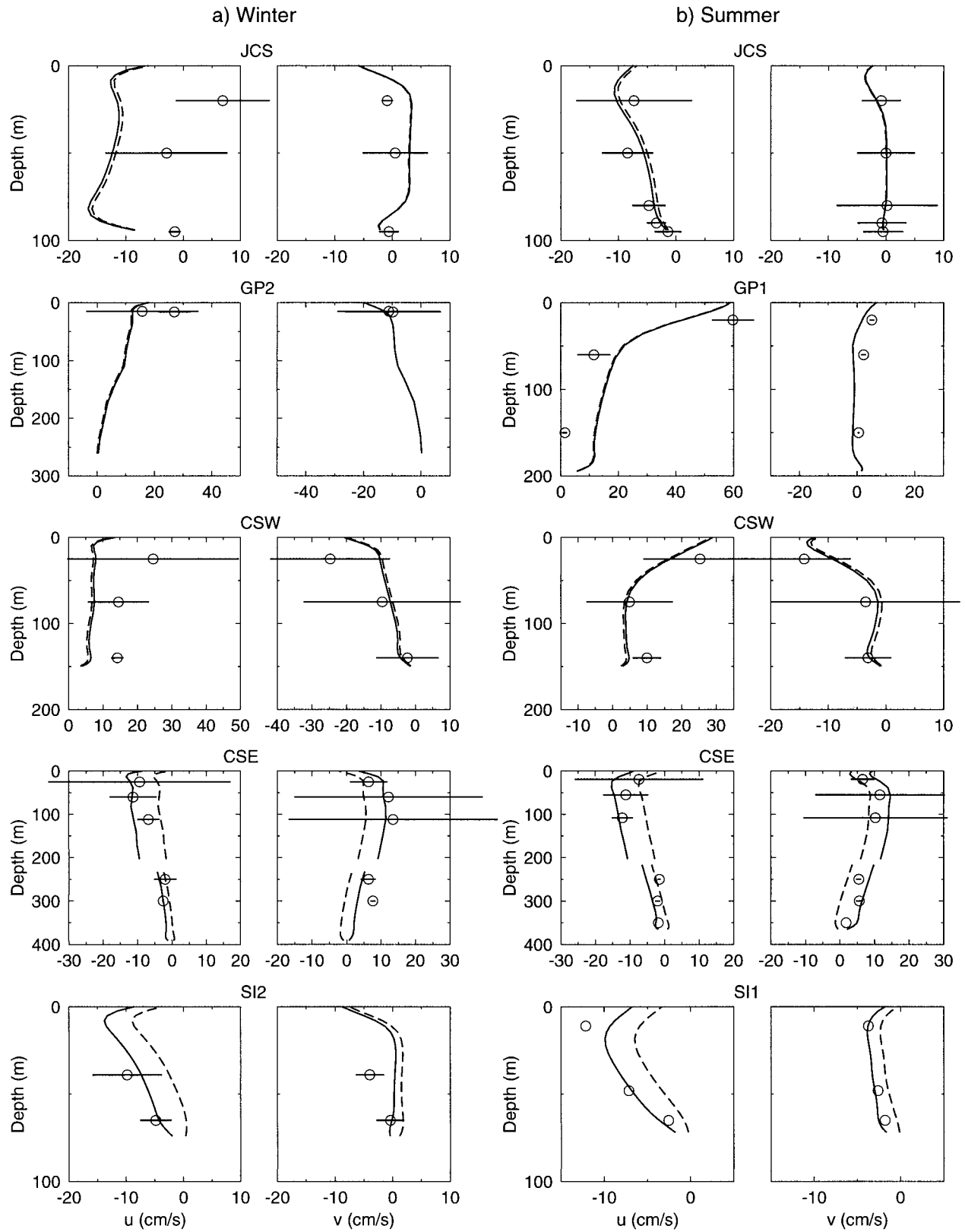
FIG. 13. Comparison of model current profiles with observed bimonthly mean currents (open circles) for (a) winter and (b) summer. Profiles from the composite base model solutions (solid curves, with additional barotropic SNS inflows) and analogous solutions without additional
