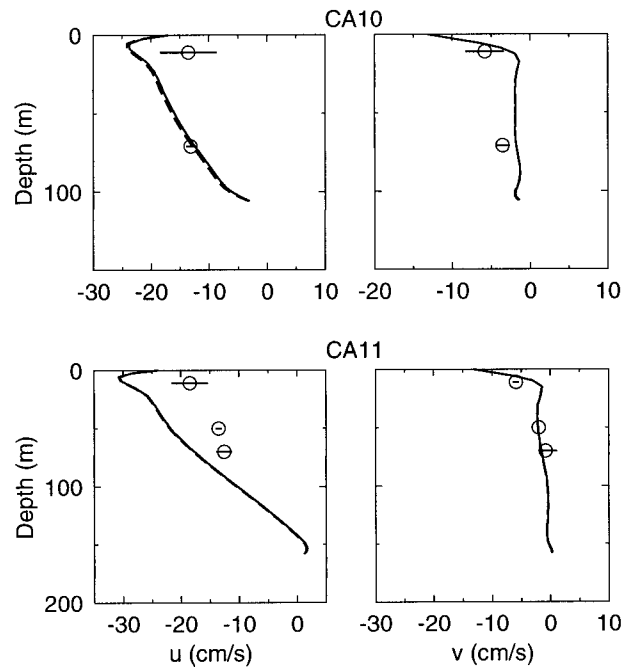
FIG. 14. Comparison of model current profiles with observed bimonthly mean currents in winter at two sites on the inner Liscomb line from the Canadian Atlantic Storms Program (CASP; Anderson and Smith 1989). Conventions as in Fig. 13.
