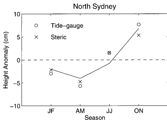
FIG. 8. Seasonal sea level anomalies at North Sydney, NS. Crosses are steric height estimates obtained from the 3D density fields, and open circles are observational estimates from tide-gauge data adjusted for inverse barometric effects. The solid line is from the model solutions with baroclinic, wind, and SBI and SNS inflow forcing.
