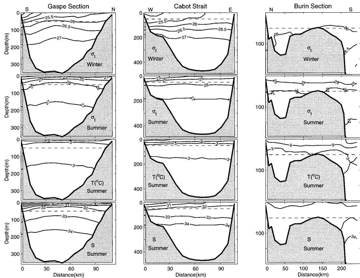
FIG. 6. Vertical distribution of density ( \sigma_t , units) on the Gaspé, Cabot Strait, and Burin sections for winter (top row) and summer (second row). The contour interval for winter is 0.5 \sigma_t units, and for summer 1.0 \sigma_t units for values of 25 and higher, and 2 \sigma_t units for lower values. Also shown are temperature (third row, with contours at 6 ^{\circ}\text{C} intervals) and salinity (bottom row, with contours at 1-psu intervals) in summer. The dashed line is the 50-m level.
