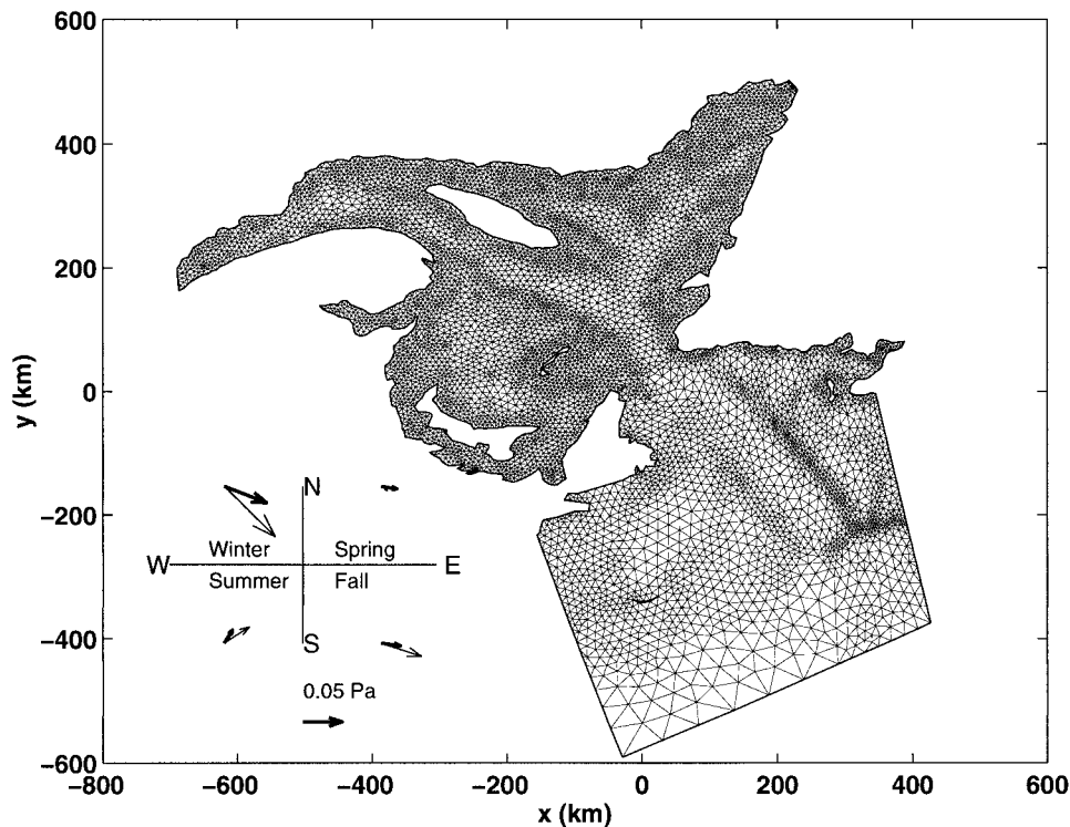
FIG. 3. The horizontal finite element grid (core3) used for the hydrographic fields and in the numerical model. The model origin is at 47^{\circ}\text{N} , 60^{\circ}\text{W} . Also shown are the magnitude and direction of the climatological seasonal-mean wind stresses at Sable Island (thick arrows) and Magdalen Shallows (thin arrows).
