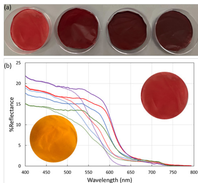
Fig. 5: (a) MR-MMM samples of MR-MOF in a PVDF matrix. From left to right the MMMs contain MR-MOF-25 (20 mg), MR-MOF-50 (10 mg), MR-MOF-75 (10 mg), and MR-MOF-100 (1 mg) in 100 mg of PVDF. (b) Reflectance measurements of MR-MOF before (low-energy onset) and after (higher energy onset) ammonia exposure. Photographic inset shows MR-MMM-25 before and after ammonia exposure. MR-MMM-25 (blue), MR-MMM-50 (red), MR-MMM-75 (purple), and MR-MMM-100 (green). Traces are boxcar averaged.
