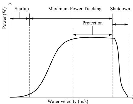
Fig. 5. Control stages of River Current Turbine
