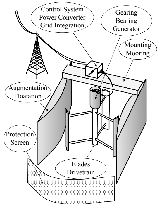
Fig. 4. River current turbine system sketch
