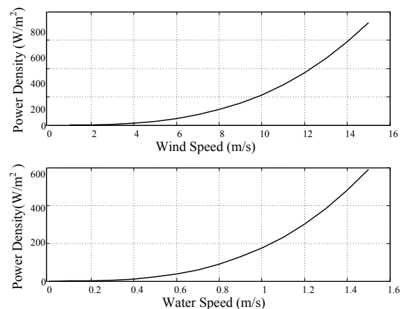
Fig. 1. Power density of wind turbine and hydrokinetic turbine
