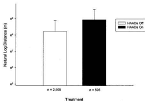
Figure 2. The natural log distance (mean ± s.d.) between HAADs and humpback and fin whale sightings by treatment condition in 1995.
