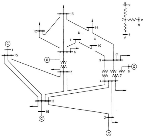
FIGURE A.1 MODIFIED IEEE 14 BUS SYSTEM
