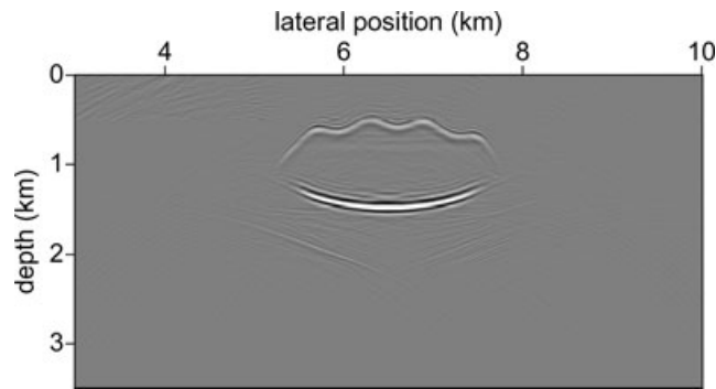
Figure 9. Imaging with underside reflections using offsets up to 6 km; the triply scattered waves propagate through the salt. This image illustrates that, under idealized circumstances, underside reflections and topside reflections can be used in a similar way in non-trivial structures.
