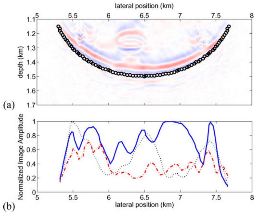
Figure 12. Amplitude extraction along the base of salt. The maximum amplitude within one wavelength of the set of points shown in (a) overlain on the image from Fig. 8(a) is plotted in (b) for each of three images. The ‘perfect’ image made with singly scattered data shown in Fig. 8(a) (solid blue line), the image, shown in Fig. 8(b) made with the inclusion-free velocity model (dashed red line) and the image shown in Fig. 10(c) made with multiply scattered waves from below the salt (dotted black line). Both primary images are normalized by the maximum amplitude in the image made with the correct velocity model; the triple scattered image is normalized to its maximum value. The lines have been smoothed with a 3-point median filter.
