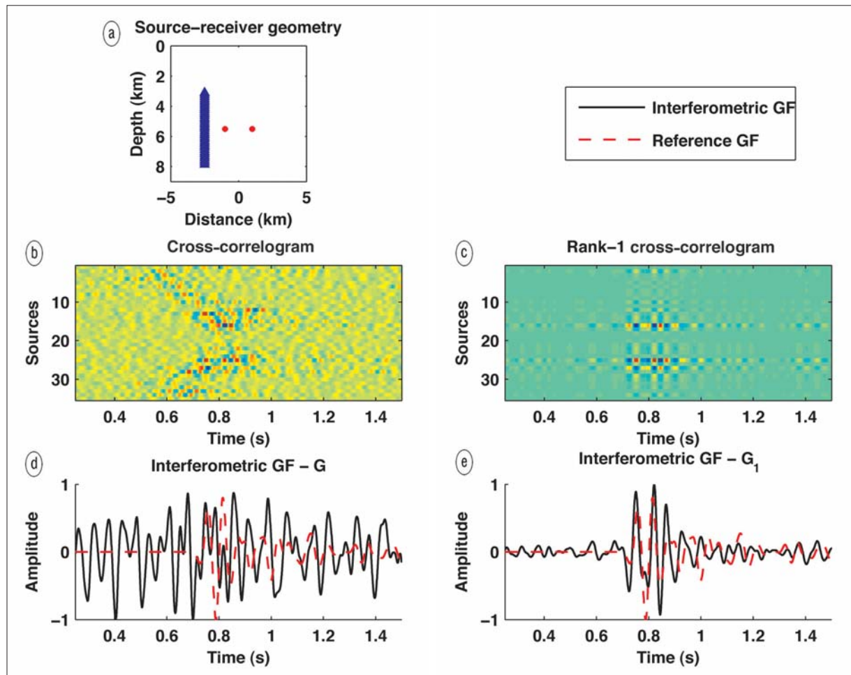
Figure 7. (a) Source-receiver geometry = one borehole with 35 receivers (blue triangles) and two microquakes (red stars); (b) original cross-correlogram; (c) rank 1 cross-correlogram; (d) standard interferometric GF, \mathbf{G} ; (e) rank 1 GF, \mathbf{G}_1 . The black line corresponds to the interferometric GFs and the red line to the true GF. In (e) the random noise is reduced to the level of the coda and the GF is clearer than in (d).
