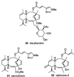
Figure 1.17 Structures of eleutheroides 50-52 .
