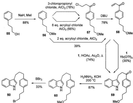
Scheme 3.15 The third attempts under Strategy D.
