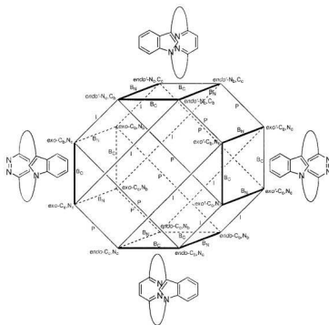
Figure 4.10 Selected conformational processes in 41 .
