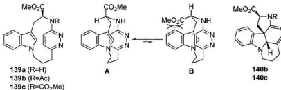
Figure 5.8 Conformational preference of cyclophanes 139a-c and the structure of products from their transannular IEDDA reactions.
