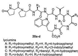
Figure 3.3 Structures of lyciumins A-D 20a-d .
