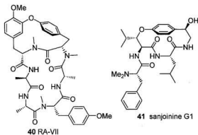
Figure 1.14 Structures of RA-VII 40 and sanjoinine G1 41 .
