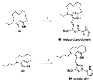
Scheme 1.12 Pyrrolophane intermediates 57 and 59 in Fjirstner's formal syntheses of metacycloprodigiosin 58 and streptorubin B 60 .
