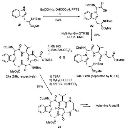
Scheme 3.7 Synthesis of lyciumins A and B.
