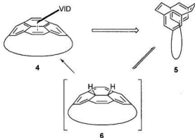
Scheme 2.1 Retrosynthetic analysis of (2,7)pyrenophane. (Part I)
