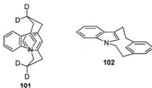
Figure 3.23 Structures of indolophanes 101 and 102 .
