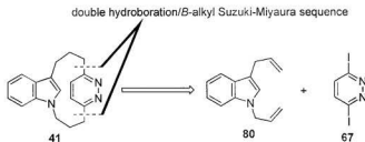
Scheme 4.24 The fifth retrosynthetic analysis of 41 .
