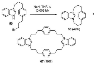
Scheme 3.17 Final ring closure of bromide 50 .
