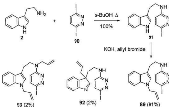
Scheme 5.14 Synthesis of cyclization precursor 89 .
