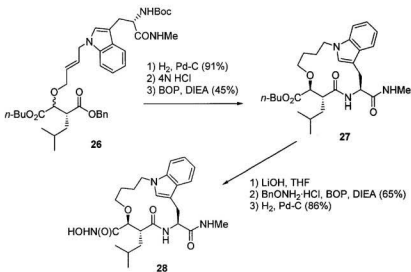
Scheme 3.8 Synthesis of indolophane 28 .
