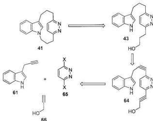
Scheme 4.18 The third retrosynthetic analysis of 41 .
