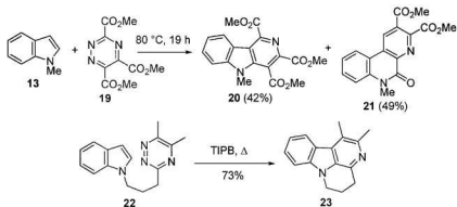
Scheme 4.5 The IEDDA reaction of indoles with 1,2,4-triazines.
