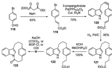
Scheme 5.25 Attempted synthesis of cyclophane 123 .
