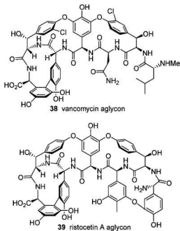
Figure 1.13 Structures of vancomycin aglycon 38 and ristocetin aglycon 39 .
