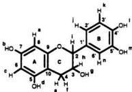
2-(3,4-Dihydroxyphenyl)-3,4-dihydro-2H-1-benzopyran-3,5,7-triol (+)-Catechin
