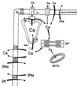
Figure 1.2 Schematic of \text{Ca}^{2+} regulating mechanisms in cardiac muscle. ATP, adenosine triphosphate; MITO, mitochondrion; MF, myofilaments; Na-CaX, \text{Na}^+/\text{Ca}^{2+} exchanger; SL, sarcolemma; SR, sarcoplasmic reticulum; \text{I}_{\text{Ca}} , L-type \text{Ca}^{2+} channel. Taken from Tibbits et al. 1991.
