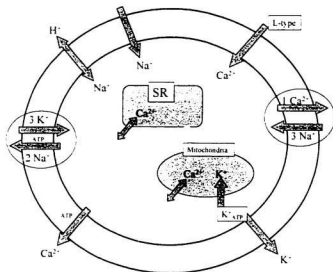
Figure 1.3 Schematic drawing of major ion fluxes and regulating mechanisms in cardiomyocytes.
