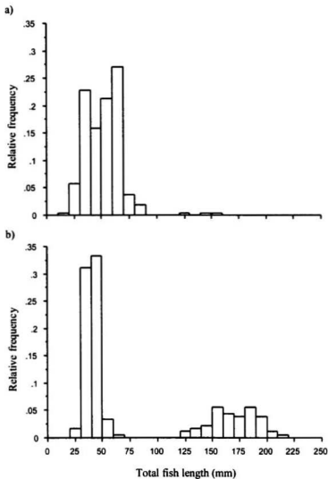
Figure 3.6 Length histograms of sand lance collected from Atlantic Puffins provisioning chicks at Gull Island in 1997 (a) and 1998 (b).
