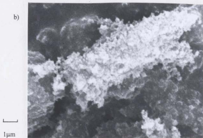
Figure 4.15 SEM Micrographs of Char Activated (a) by Steam and (b) by CO 2
