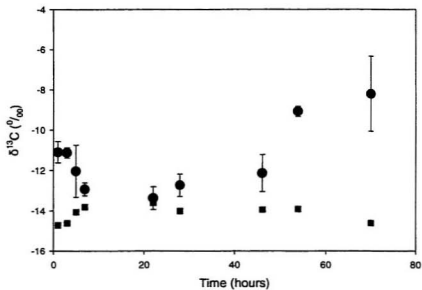
Figure 13: Isotopic Fractionation of t-DCE over Time. The circles represent data from the reaction vessels, and the squares represent the t-DCE blank (solvent and water only).
