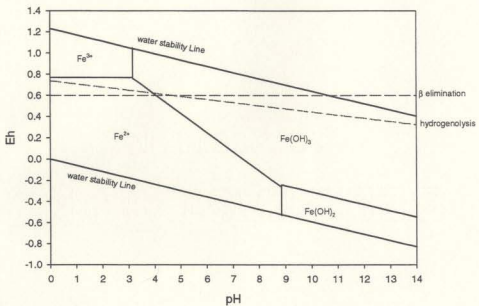
Figure 21: Phase Diagram for Iron Hydroxide Species and TCE Reductive Dehalogenation Reactions (after Brookins, 1988). The dehydrogenation product is cis-DCE. Data for the dehalogenation was calculated from Roberts et al. (1996).
