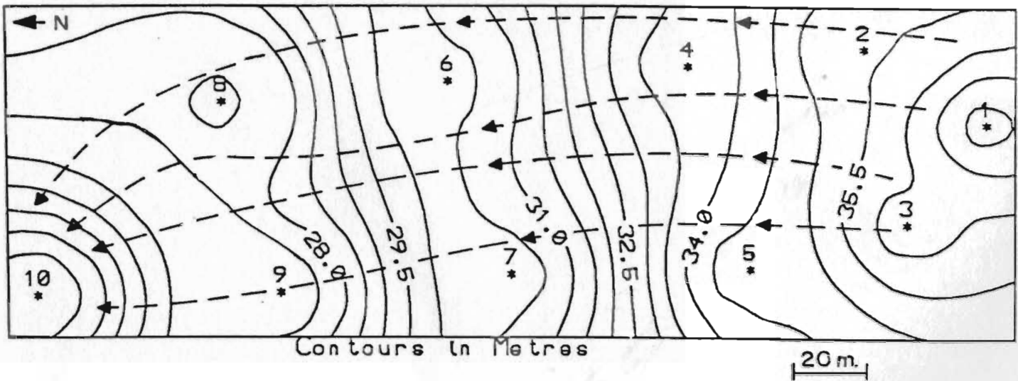
B. High Water Table Contour - April 26, 1991
