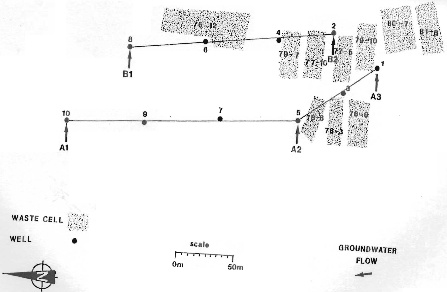
Figure 3.3 Location of two geologic cross-sections.
