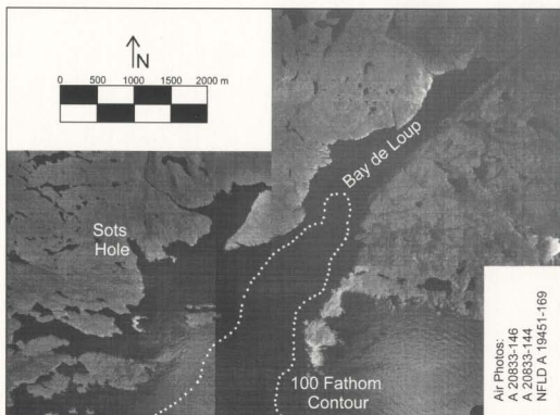
Figure 3-6 Bay de Loup
