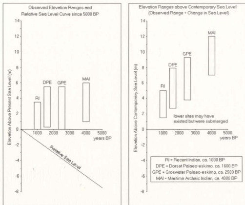
Figure 5-1 Ranges in site elevations above present and contemporary sea levels. The left side illustrates the elevations of the sites as they were recorded. The right side illustrates the original elevation of the sites above their contemporary sea level.
