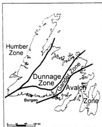
Figure 3-1 Tectonic Zones of Newfoundland (after Rogerson 1981)
