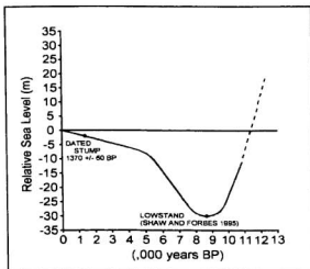
Figure 3-2 Preliminary relative sea level curve for Burgeo
