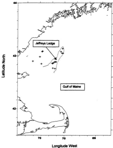
Figure 3.12: Spatial distribution of observed harbour porpoise incidental capture in fixed gillnets placed in waters adjacent to Jeffreys Ledge in the Gulf of Maine during 1993.
